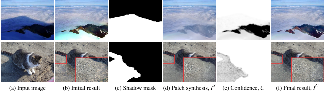
Figure 2: Given an input image I (a), we compute an initial shadow removal result, I^N (b) using current shadow removal methods (top, [LG08], bottom, [MM10]). We use this result to estimate a shadow mask (c), and a patch-based synthesized image, I^S (d). This result is inaccurate in regions that are not observed in the non-shadow region and this is captured by the confidence map, C (e). Combining I^N and I^S using C gives us the final correction, I^C , (f) where the inconsistency artifacts in I^N are removed.
